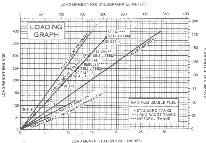
Figure 6-6. Loading Graph
