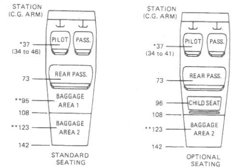
Figure 6-3. Loading Arrangements
